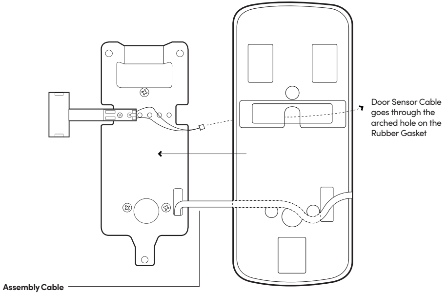
Right-hand Installation
